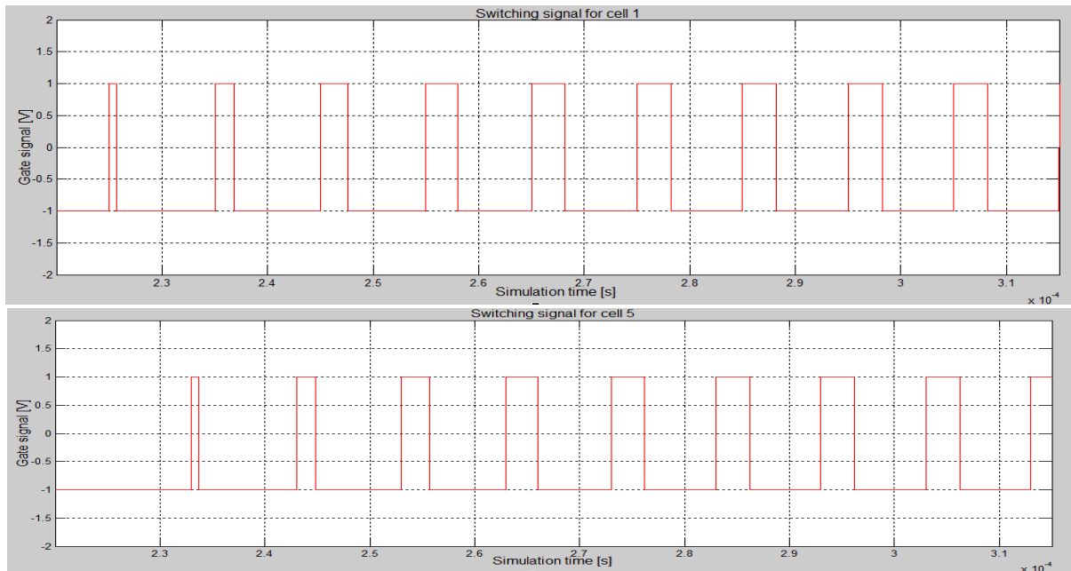
Figure 8: Switching mechanism for 5 phases buck converter
