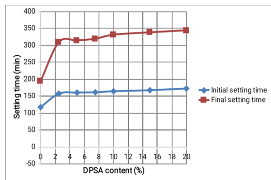
Figure 1: Setting times of cement-DPSA paste for cement replacement
