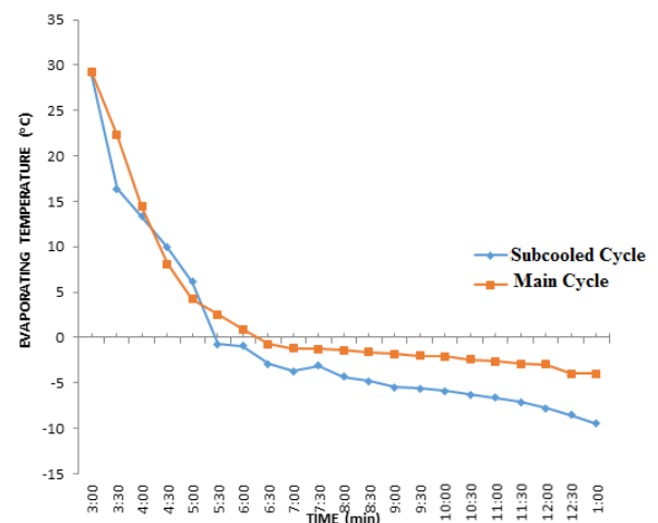
Figure 7: Variation of evaporating temperature with time
