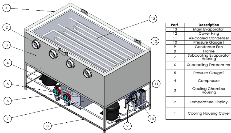
Figure 2: Isometric view of the designed freezer-type subcooled vapour compression refrigeration system
