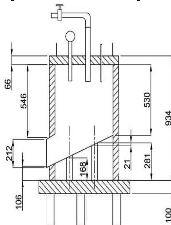
Fig. 2: Sectional view of steam cooking chamber
