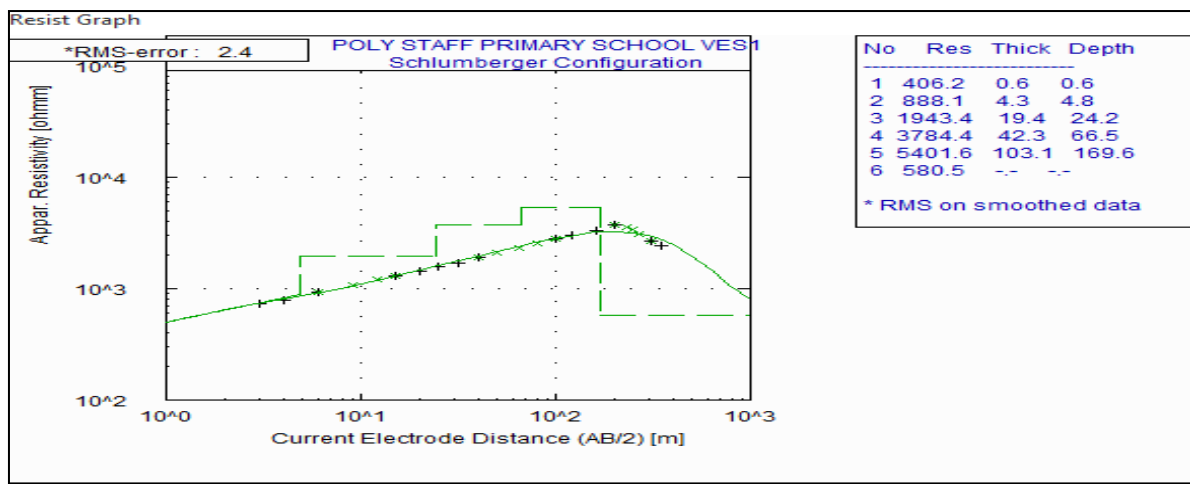
Figure 3: Resistivity curve for VES 1
