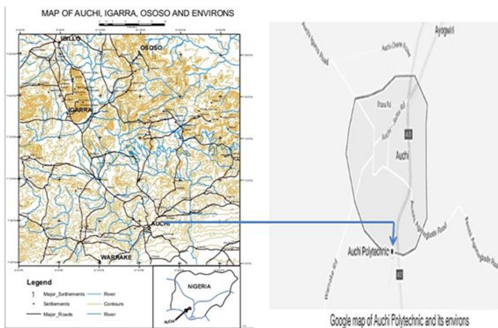
Figure 1: Geophysical map of Auchi [11]
