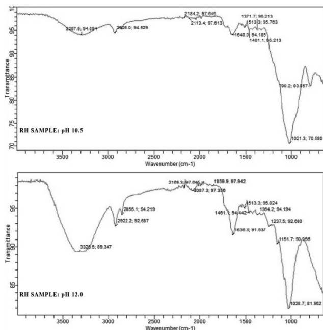
Figure 3: FTIRS Spectrum for pH levels 10.5 and 12.0 Treated RHS
