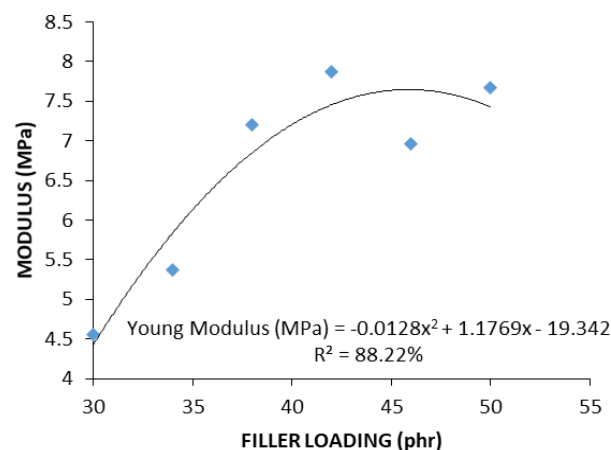
Figure 5: Tensile modulus of the RHA-NR composites
