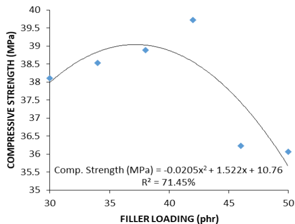
Figure 4: Compressive strength of the RHA-NR composites
