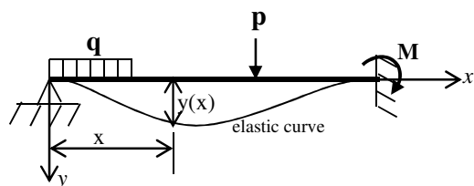
Fig.1 Beam element under generalized load
