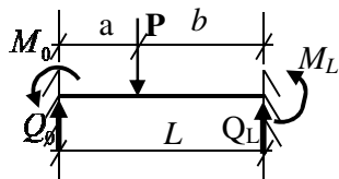
Fig.6: Fixed ended beam with a point load
