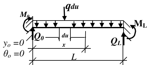
Fig.8 :Fixed ended beam with uniformly distributed load
