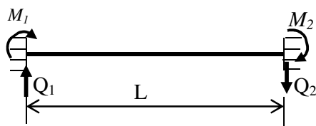
Fig.9 Fixed ended beam element
