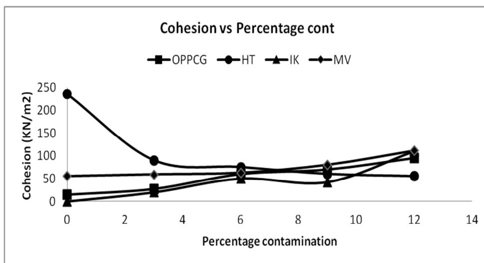
Fig 7: Graph of Cohesion vs. Percentage contamination
