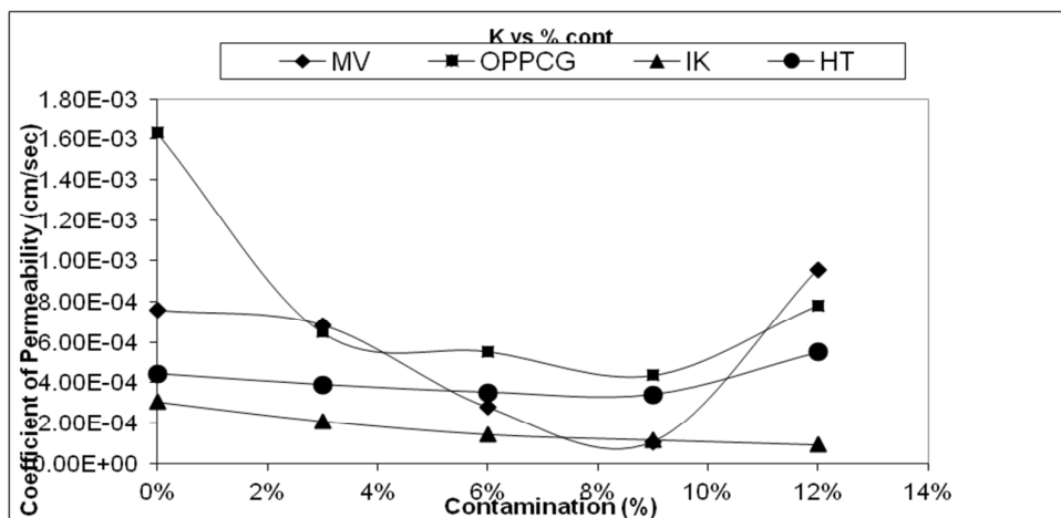
Fig 6: Graph of Coefficient of Permeability vs. Percentage contamination
