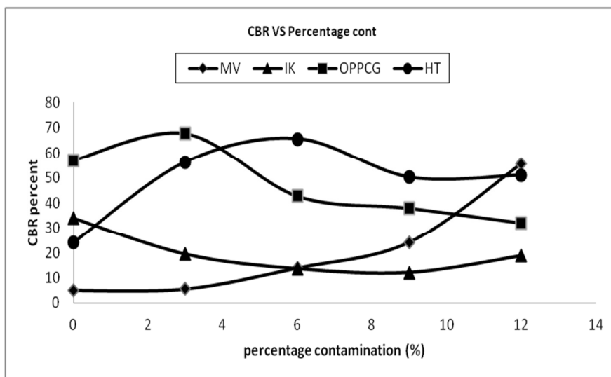
Fig 9: Graph of CBR vs. Percentage Contamination
