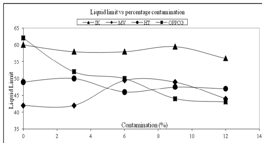
Fig 2: Graph of Liquid limit vs. percentage contamination
