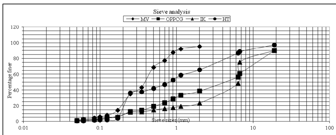
Fig 1: Sieve analysis of the soil samples
