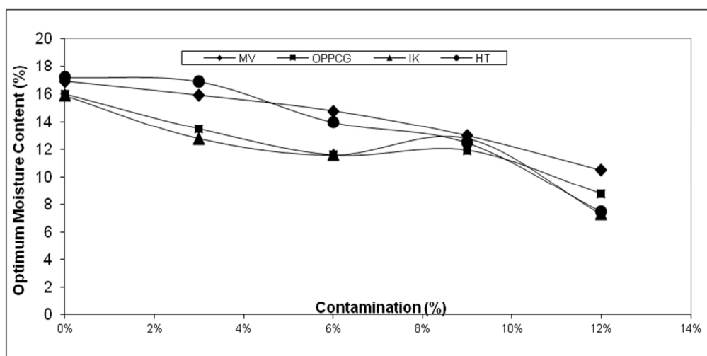
Fig 4: Graph of Optimum moisture content vs. Percentage contamination
