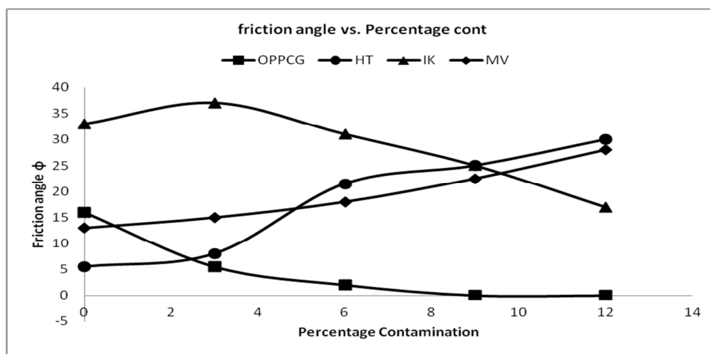
Fig 8: Graph of Friction angle vs. Percentage contamination
