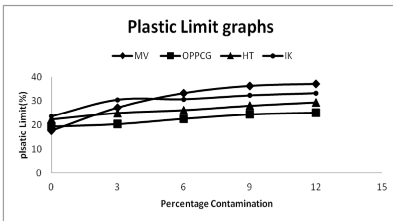
Fig 3: Graph of plastic limit vs percentage contamination
