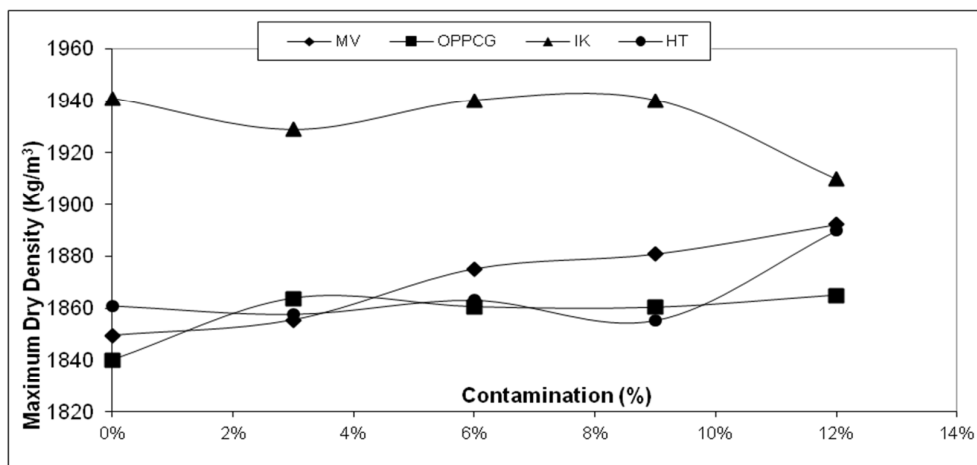
Fig 5: Graph of maximum dry density vs. percentage contamination
