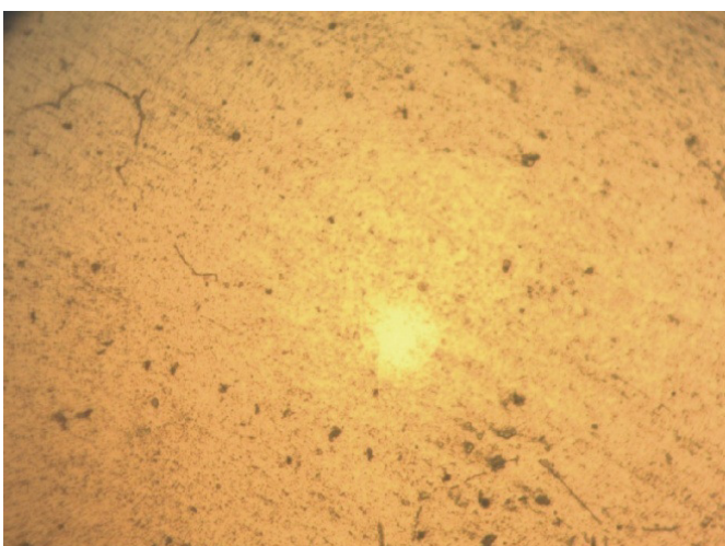
Figure 2: Micrograph of Al-12wt%Si + 0.02% S alloy casting (200x).
