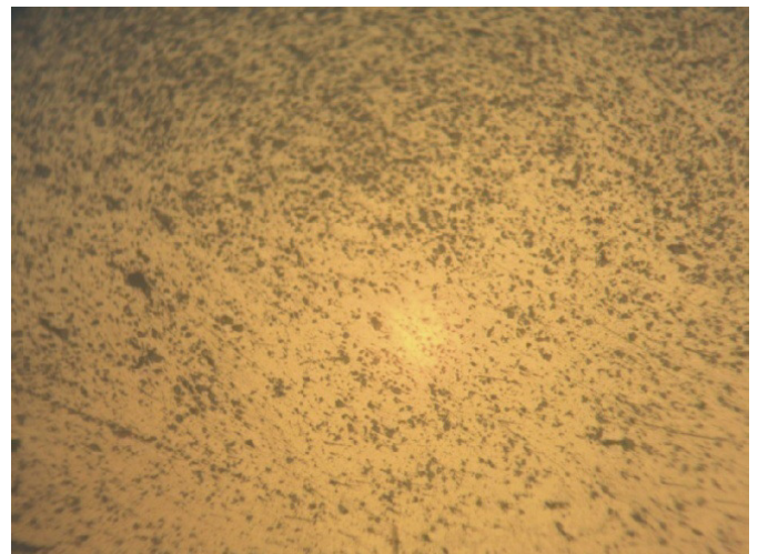
Figure 5: Micrograph of Al-12wt%Si + 0.1% S alloy casting (200x).
