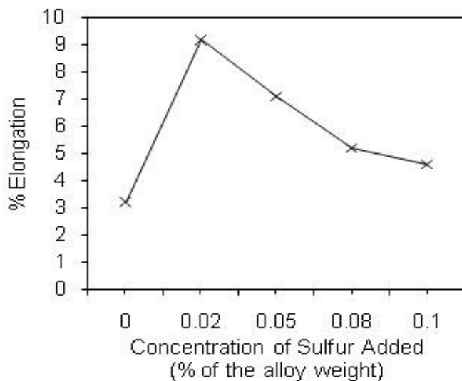
Figure 8: Variation of % Elongation of Al-12wt%Si sand cast alloy with sulphur addition.
