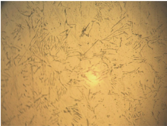
Figure 1a: Micrograph of unmodified Al-12wt% Si alloy casting (200x).
