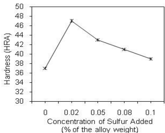
Figure 7: Variation of Hardness of Al-12wt%Si sand cast alloy with sulphur addition.
