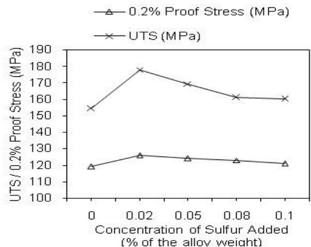
Figure 6: Variation of UTS/0.2% Proof Stress of Al-12wt%Si sand cast alloy with sulphur addition.
