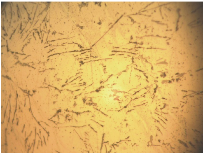
Figure 1b: Micrograph of unmodified Al-12wt% Si alloy casting (400x).
