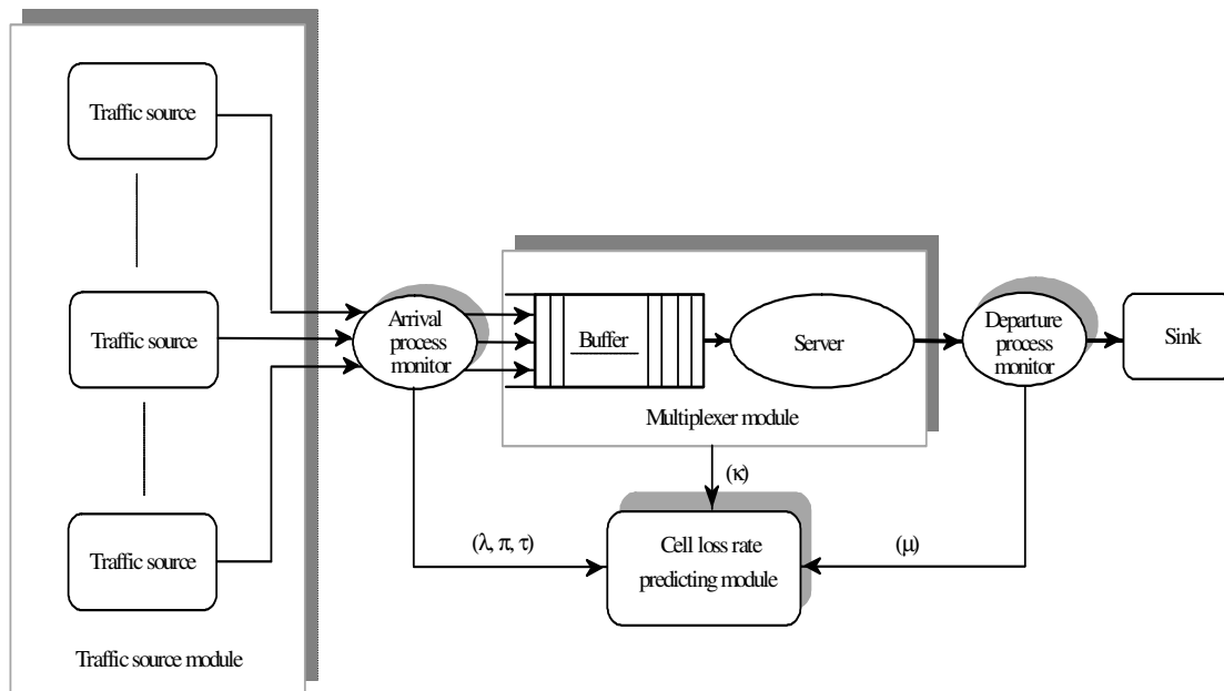
Figure 1: Integrated simulation model
