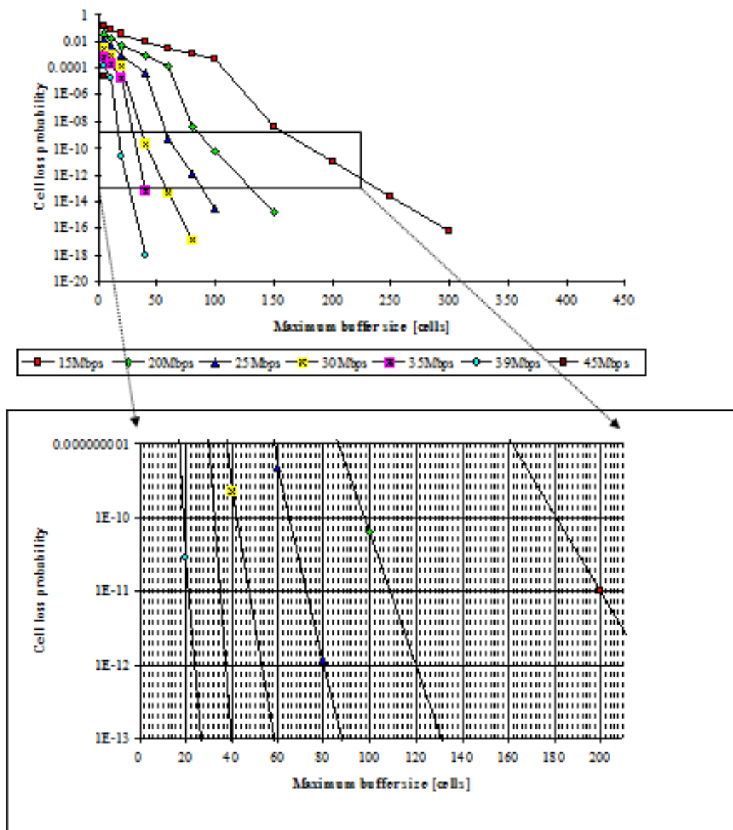
Figure 2: Data traffic cell loss rate as a function of buffer size at various bandwidths for 5 sources
