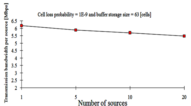
Figure 5: Statistical multiplexing gain
