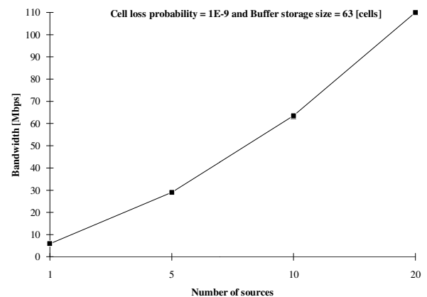
Figure 4: Data traffic resource allocation curve
