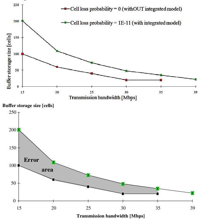
Figure 3: Comparison between integrated and traditional simulation model for data traffic sources = 5
