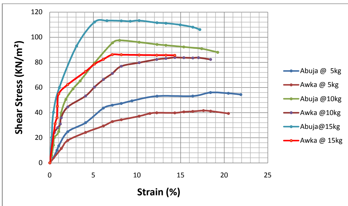
Figure 9: Determination of unconfined compressive strength in the sampled soils.
